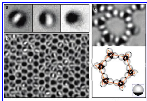
Figure 3. Triblock spheres visualized by bright-field optical microscopy. (a) Images of an individual sphere with X-shaped surface functionalization. Metal patches appear black and silica patches appear white, showing the particle orientation. (b) Example of a hexagonal lattice formed by these symmetric triblock, X-type silica spheres in deionized water, the poles being hydrophobic and the middle band charged. (c) Example of the dodecagonal pore of a truncated hexagonal lattice formed from triblock silica spheres with Y-shaped bonding geometry, where the gold patches were rendered hydrophobic via thiol chemistry.
