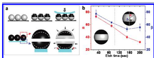
Figure 1. Synthesis of triblock spheres. (a) Parent colloidal spheres on a flat substrate are first coated on one hemisphere with 2 nm Ti and 25 nm Au (black), then pressed against a sticky PDMS stamp to release the uncoated hemisphere, flipped over, and decorated with the same coating again. The stamp is subsequently immersed in a gold-etching solution. The gold coatings on the top and bottom shrink differently. (b) The angles \alpha and \beta (defined in the inset) are a measure of the size of the top (red circles) and bottom (blue squares) gold patches, respectively. Plotted against etch time, they illustrate how these patches etch at different rates.
